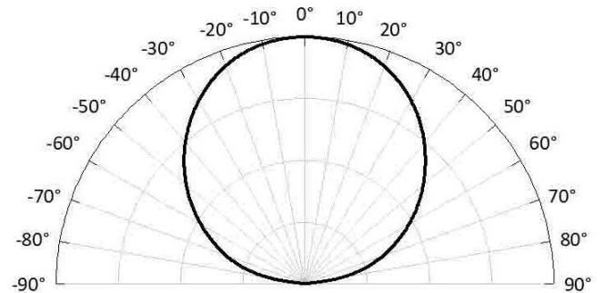
Radiation Pattern
