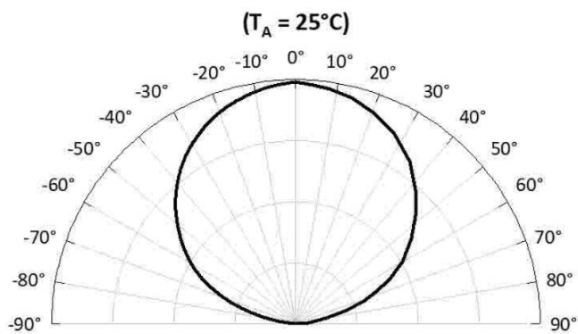
Radiation Pattern
